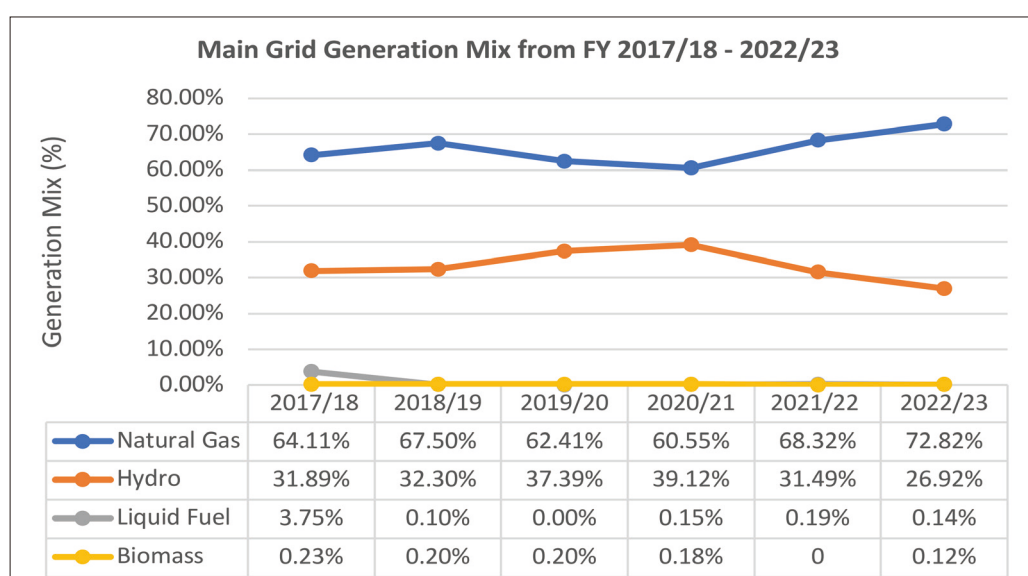
Figure 5: Energy Generation Mix (%) from FY 2017/18 – 2022/23
