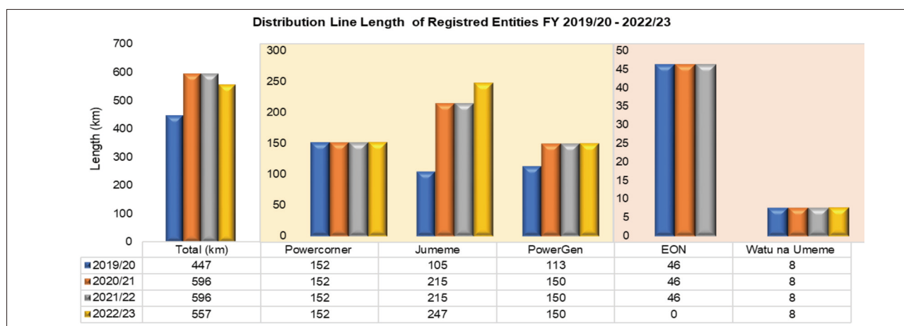
Figure 17: Distribution Line Length of Registered Entities FY 2019/20 – FY 2022/23
